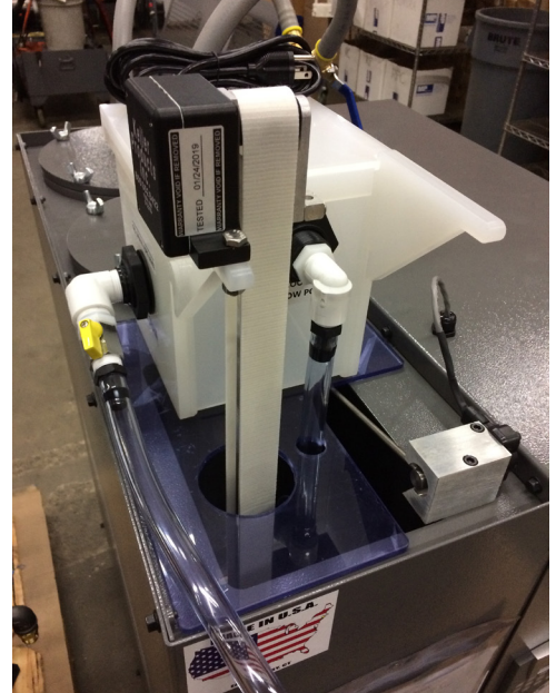
Keller Skimmer package fits directly onto tank opening.
